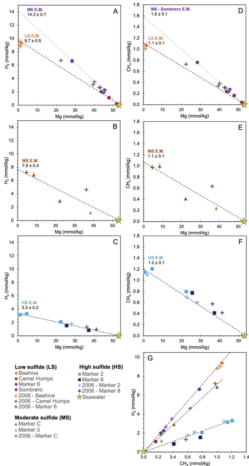
Fig. 10. Measured and endmember volatile compositions at LCHF. (A-C) Measured \text{H}_2 concentrations plotted against measured Mg define three separate mixing lines for each of the vent group (low, moderate, and high sulfide groups). This suggests that there are at least three endmember \text{H}_2 compositions at LCHF. (D-F) Measured \text{CH}_4 concentrations against Mg for each of the vent groups. Except for those calculated from the Marker 6 mixing line, endmember \text{CH}_4 compositions are within a narrow range between 1.1 and 1.2 mmol/kg. Unlike those defined by sulfur chemistry (Fig. 6), mixing between seawater and Marker 6, instead of Beehive, can explain the volatile composition of the low sulfide vent group. (G) Measured \text{H}_2 and \text{CH}_4 concentrations are strongly correlated within each vent group suggesting a common flow path for each group. Symbols indicated as crosses (+) are data from Proskurowski et al. (2006). ^{87}\text{Sr}/^{86}\text{Sr} data are not available for all samples, thus, measured concentrations are plotted against Mg.
